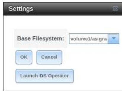
Fig. 10.3: Asigra settings
