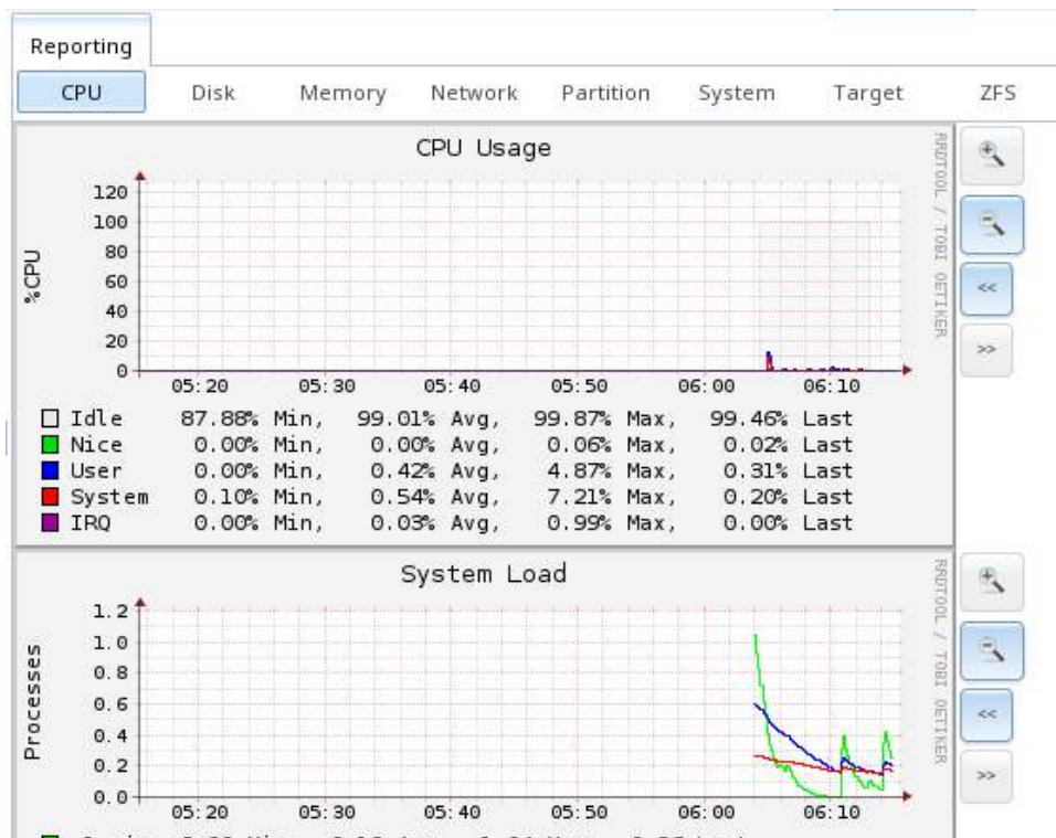
Fig. 12.1: Reporting Graphs
