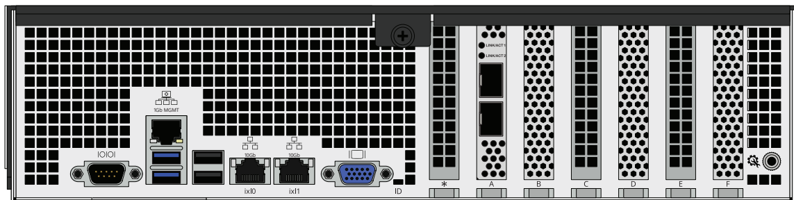
M40 Controller Expansion Slots
